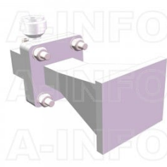
LB-90-10-C-NFSP0 Standard Gain Horn Antenna 8.2-12.4GHz 10dB Gain N Type Female
